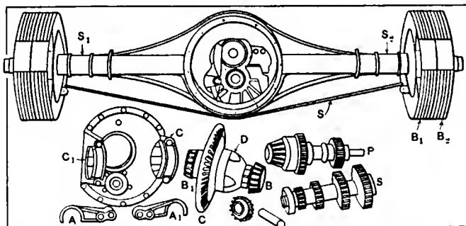
Fig. 13—Showing the Marmon transmission and differential disassembled
